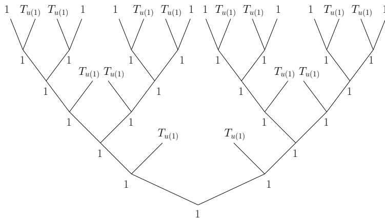
Figure 3: Tree for T_{u(2)} with Additional Nodes Pictured
