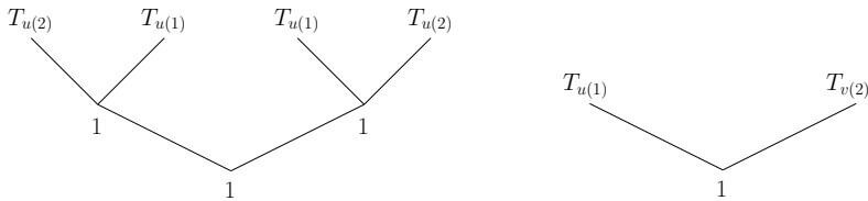
Figure 2: Trees for T_{u(2)} (left) and T_{v(2)} (right)
